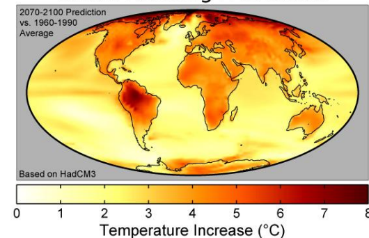
Global Warming Predictions
